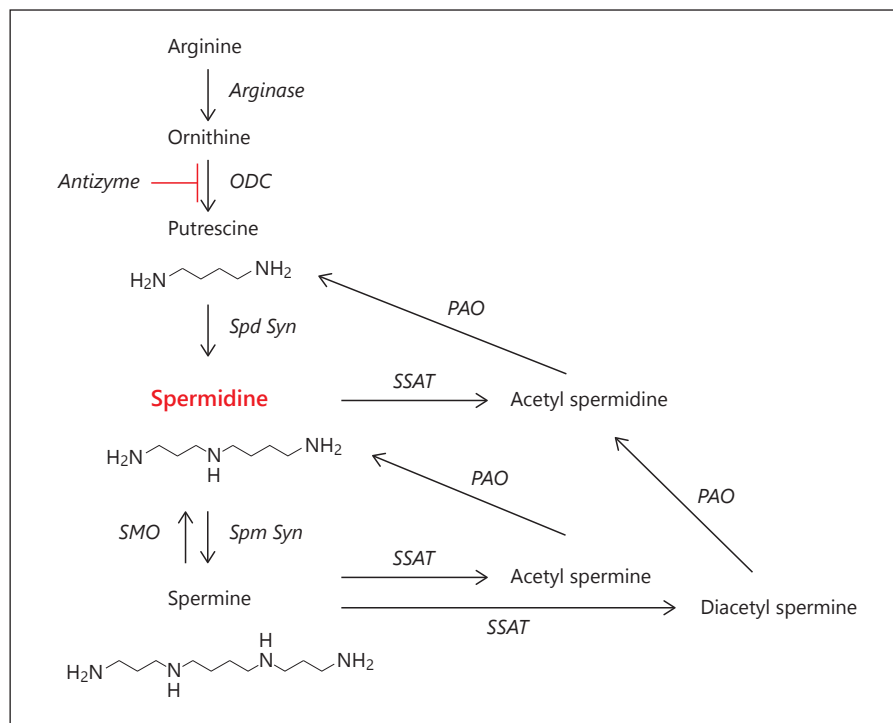
Fig. 1. Polyamine metabolism. ODC = Ornithine decarboxylase; PAO = polyamine oxidase; SMO = spermine oxidase; Spd Syn = spermidine synthase; Spm Syn = spermine synthase; SSAT = spermidine/spermine N 1 -acetyltransferase [for more details, see 1]. The levels of polyamines in many mammalian tissues are in the order spermidine > spermine > putrescine, with the ratios between them easily varying from 2 to 20.
