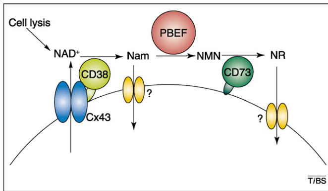
Figure 4. A potential extracellular NAD + -cycle in vertebrates. Extracellular NAD + could be derived from either cell lysis or, potentially, specific transport through Connexin 43 hemichannels. Extracellular cADP-ribose synthases, such as CD38, produce Nam from NAD + . Nam might be converted to NMN by PBEF (Nam phosphoribosyltransferase) with subsequent dephosphorylation to NR by CD73. Nam and NR are thought to be imported by unidentified transporters.
