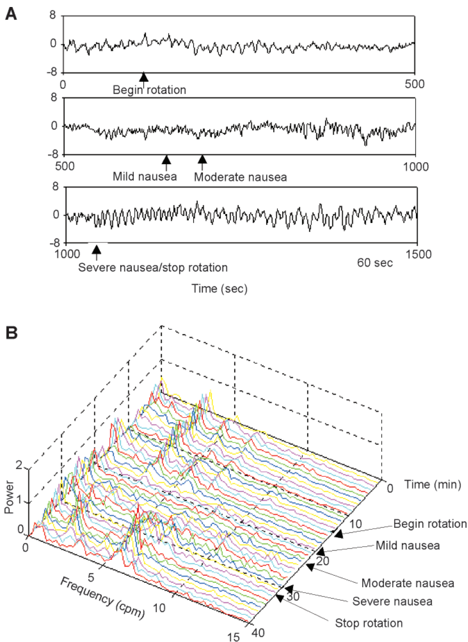
Fig. 2. Raw electrogastrographic (EGG) signals and running spectral analysis of waveform measured while a subject underwent circularvection under control conditions. A : the slow wave exhibited an oscillation of 3 cycles/min (cpm) at basal. At 540 s after initiation of drum rotation, the subject reported mild nausea, which was preceded by slow-wave disruption. At 850 s after vection was initiated, severe nausea developed accompanied by tachygastric. Tachygastric persisted after vection cessation. B : spectral analysis of the raw EGG signal. Before vection, the slow wave exhibited a dominant frequency of 3 cpm. During vection, 3 cpm were lost associated with a gradual increase in signal activity in the tachygastric range, particularly at 6 cpm; the severity of nausea increased concurrently in this period.
