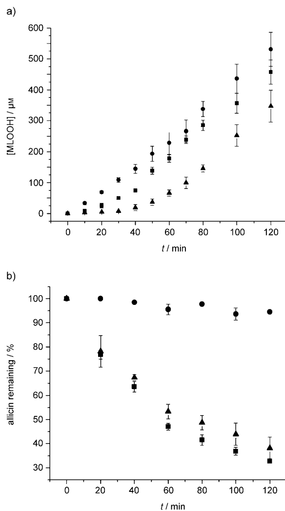
Figure 1. a) Thermally initiated (azobisisobutyronitrile (AIBN), 40 mM) autoxidation of methyl linoleate (91 mM) at 37°C in chlorobenzene containing allicin (50 \mu\text{M} ) and HFPA (0.15 M, ●), \text{CH}_3\text{CN} (1 M, ■), or no additive (▲). b) Decomposition of allicin (50 \mu\text{M} ) at 37°C in chlorobenzene containing HFPA (0.15 M, ●), \text{CH}_3\text{CN} (1 M, ■), or no additive (▲).
